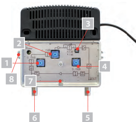
Fig. 2: HVB 31 amplifier, interior view
