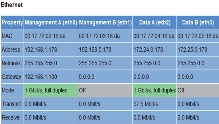
Figure 15: Status display - Ethernet
