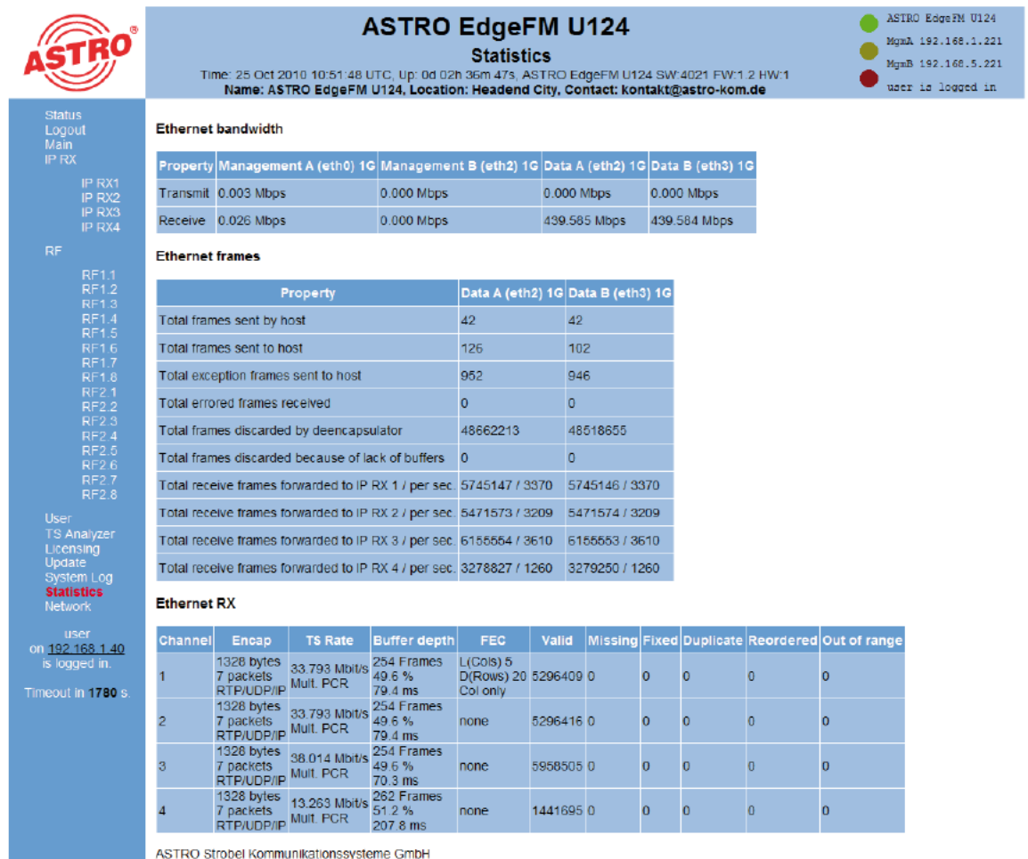
Figure 24: Statistics for the data transfer
